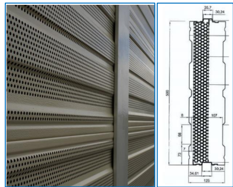
New opaque panels thicker and more absorbent to be installed
